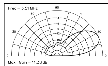
Fig A—80-meter quad elevation pattern at 3.51 MHz, at 100 feet above flat, average ground, including losses in the copper wire elements and Q = 250 inductor loading.
